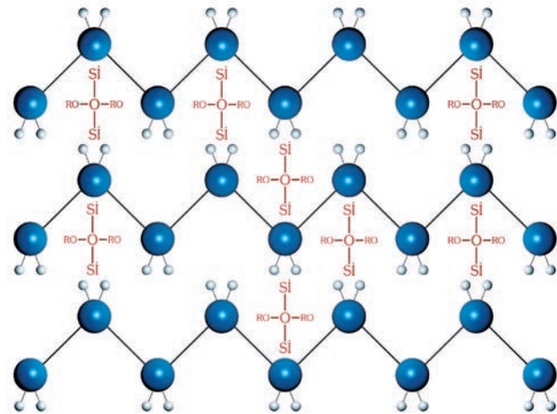
PE-Xb with cross-linking
